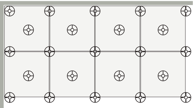
Posa sopraelevata 60x60 ± 2 cm 24"x24" ± 3/4" Installation onto flat surfaces (raised laying)
