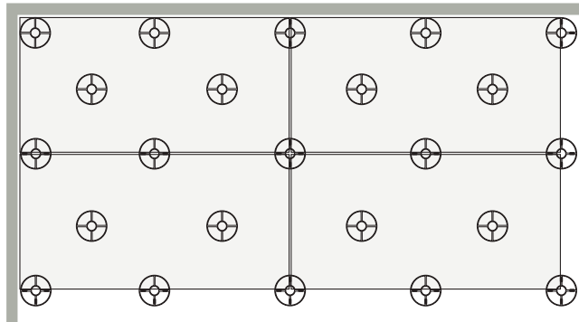
Posa sopraelevata 60x90 ± 2 cm 24"x36" ± 3/4" Installation onto flat surfaces (raised laying)
