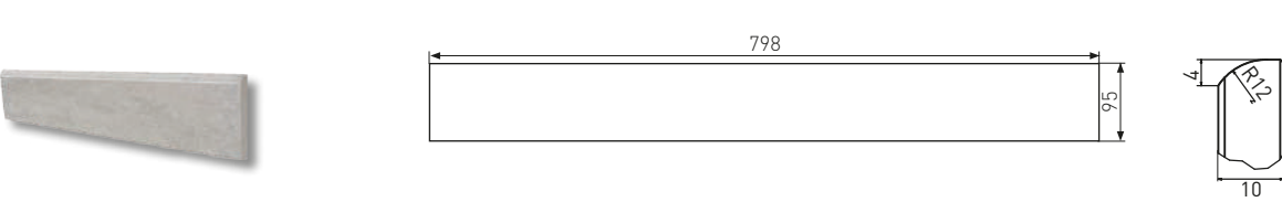
Sockel | skirting plinth | DSA89... | 798×95×10 mm
